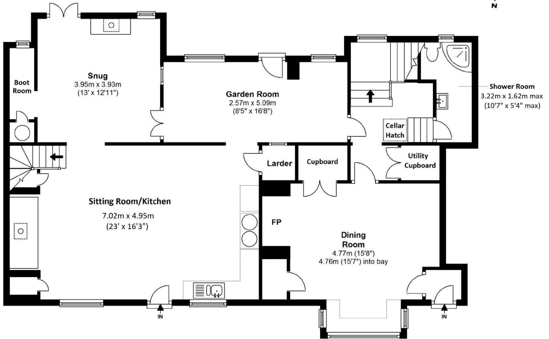
Ground Floor
