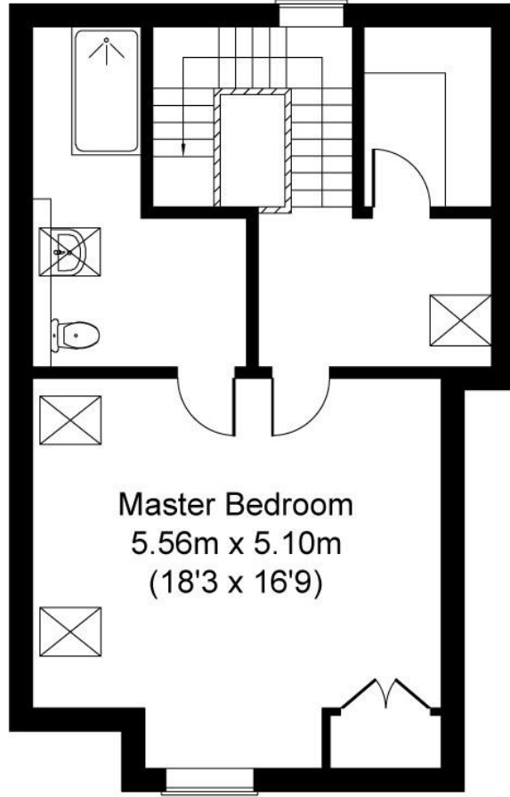
Second/Lower Roof Plan
