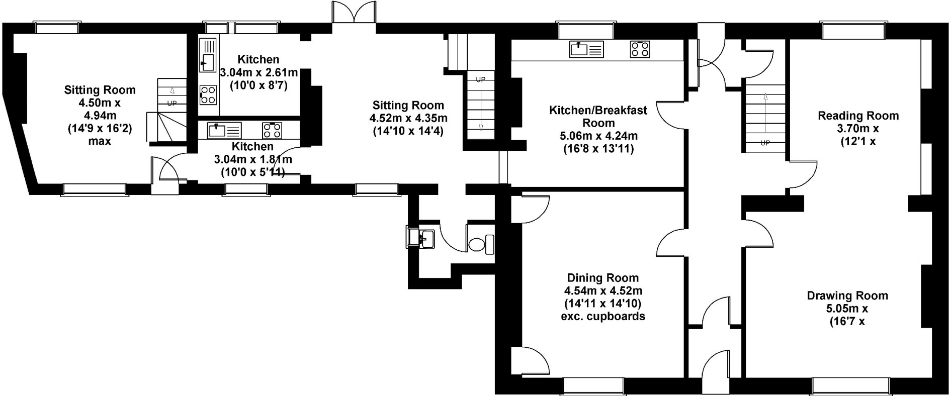
GROUND FLOOR
